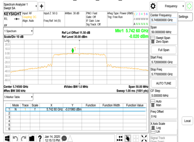
802.11ax_20MHz_Chain0_5745MHz_RU26_0
