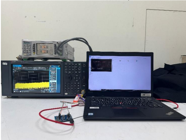
5G WLAN_Conducted_Setup
