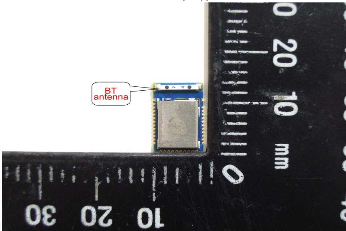
Antenna (Chip)
