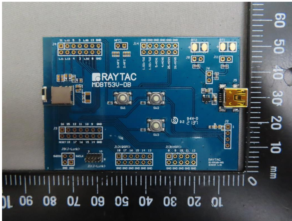
Side View of EUT_MDBT53V
