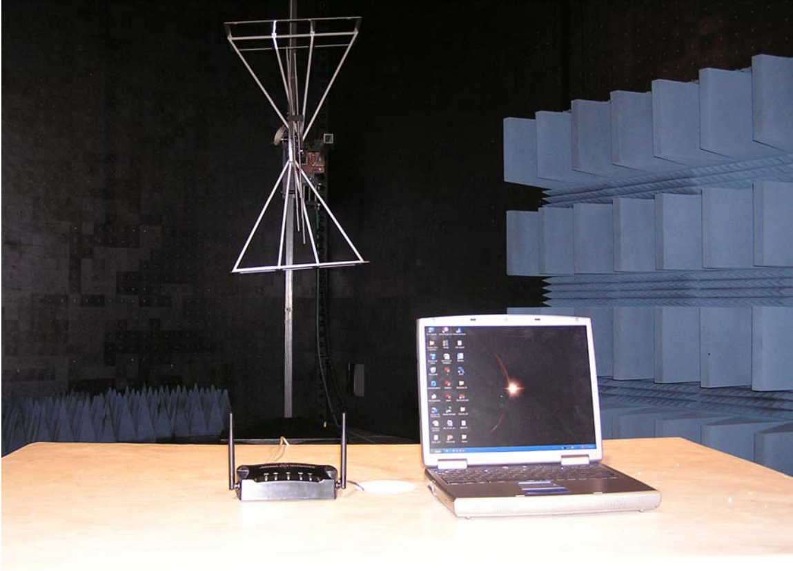
Test setup – Radiated Emissions
