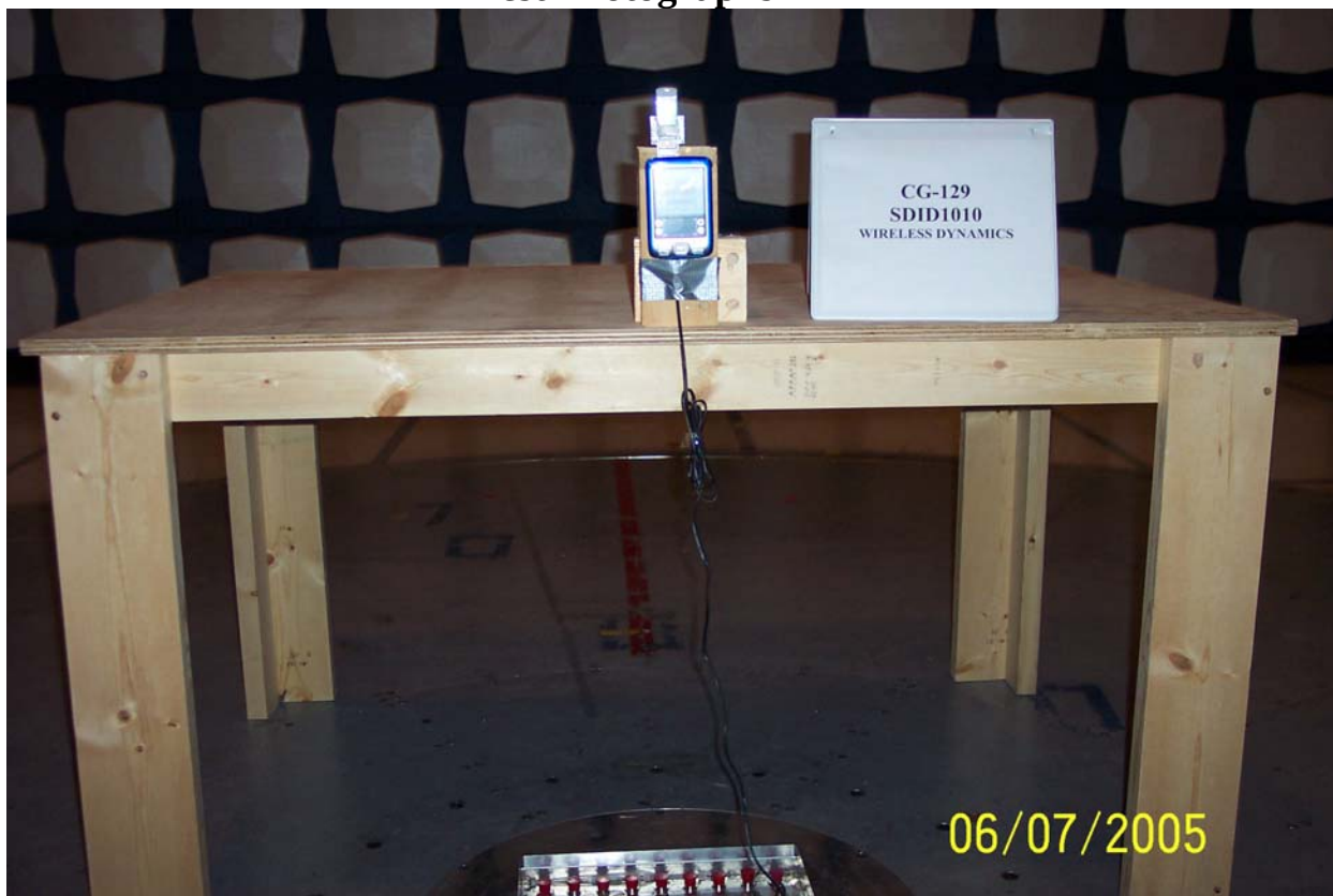
Figure 1 Radiated Emissions Test Photograph
