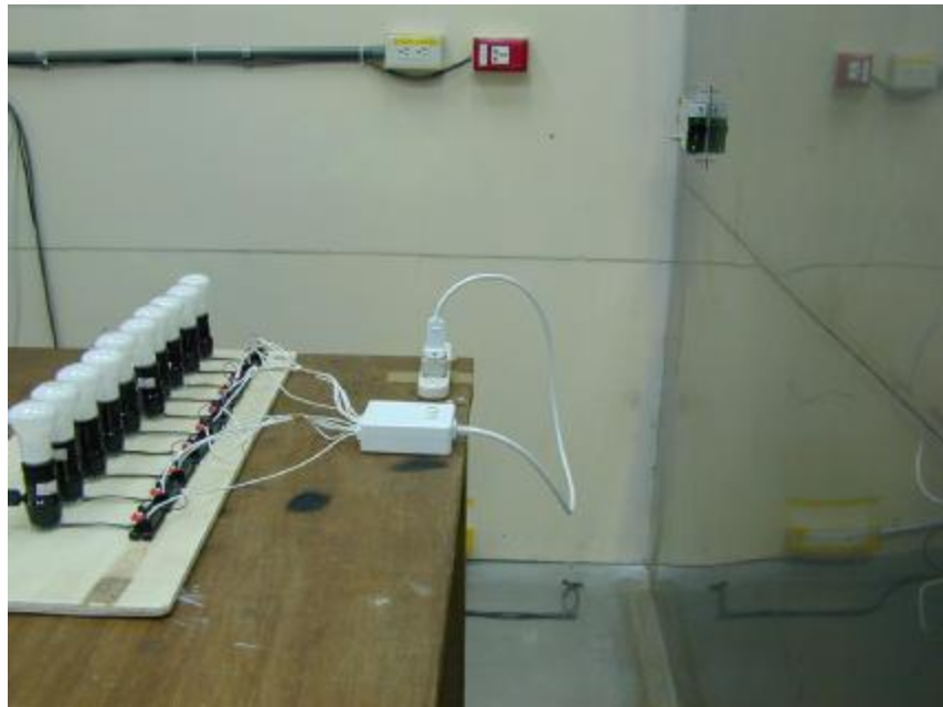
Photo 4: Conducted Emission Test Set-up (WL-905)
