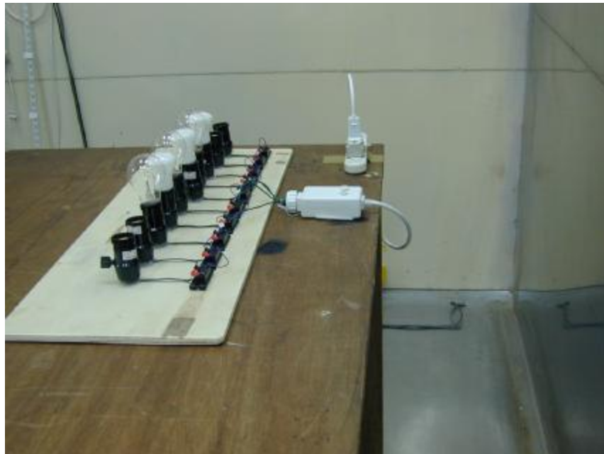
Photo 2: Conducted Emission Test Set-up (WL-902)
