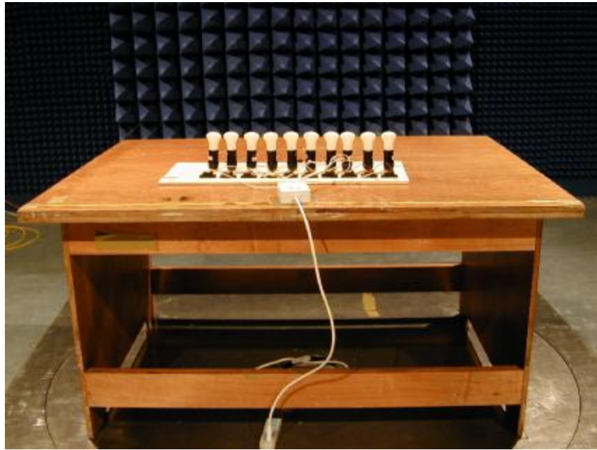
Photo 5: Radiated Emission Test Set-up (WL-905)
