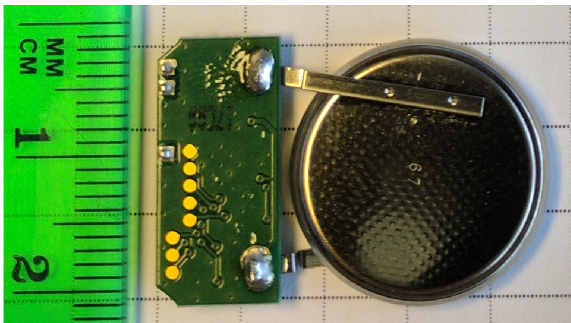
Figure 6 Interior Bottom
