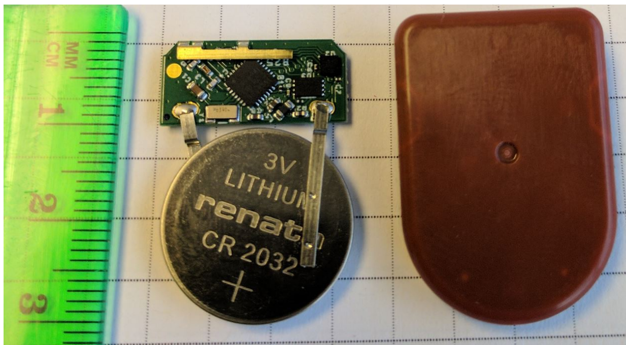
Figure 5 Interior Top
