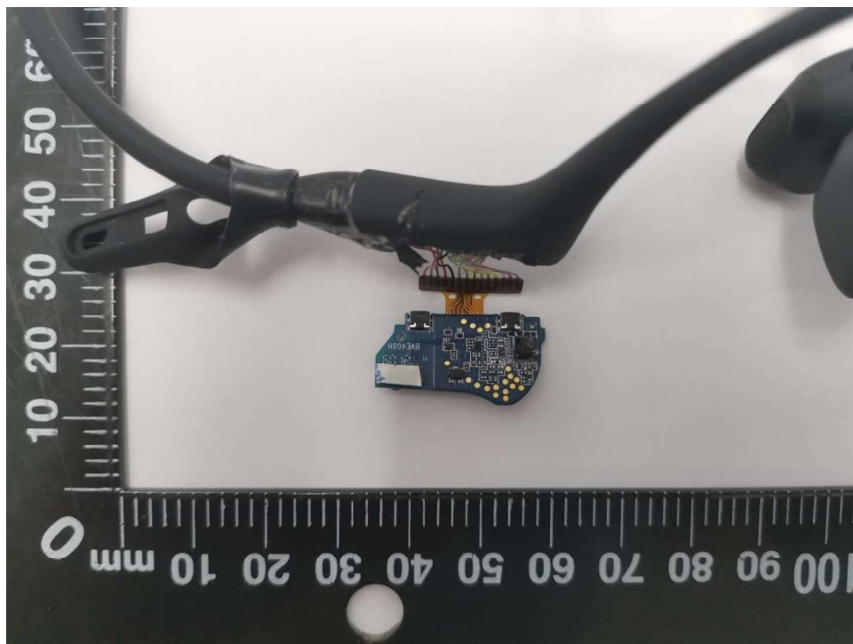
Figure 6: PCB view 2
