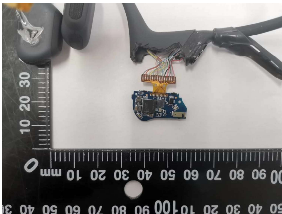
Figure 5: PCB view 1
