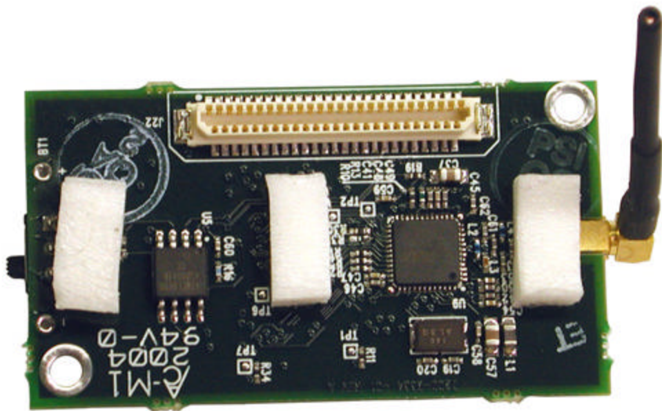
Circuit Board – Side 2
