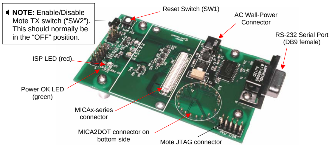
Figure 13-1. Photo of top view of an MIB510CA.
