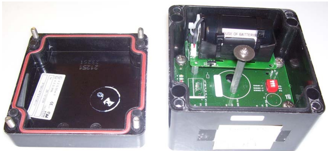
Photograph 1. Crossbow MTP400CA (8350 – 0391-01)
