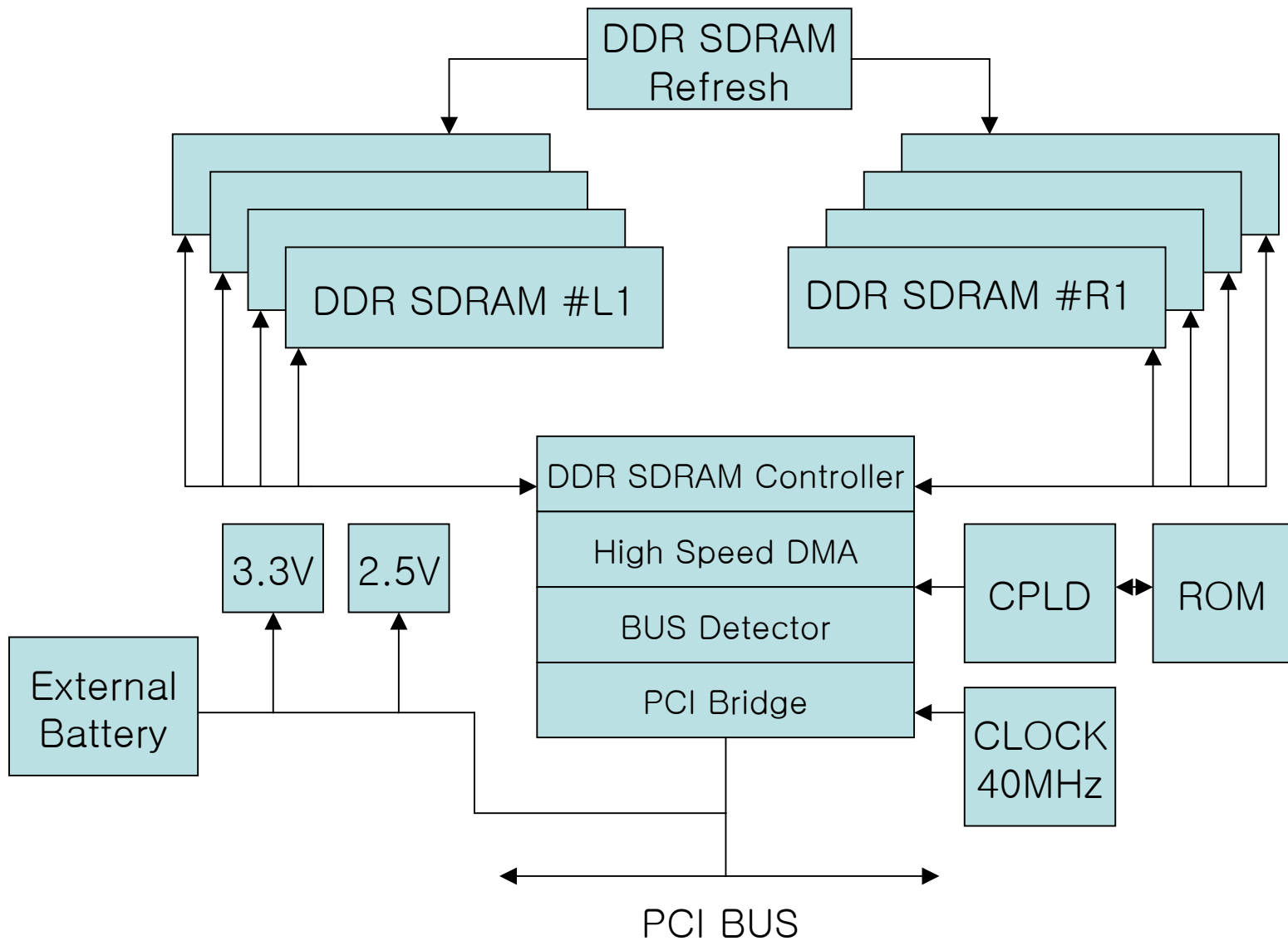
Jet-Speed Block Diagram
