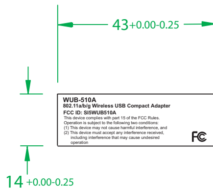
WUB-510A_Bottom Label
