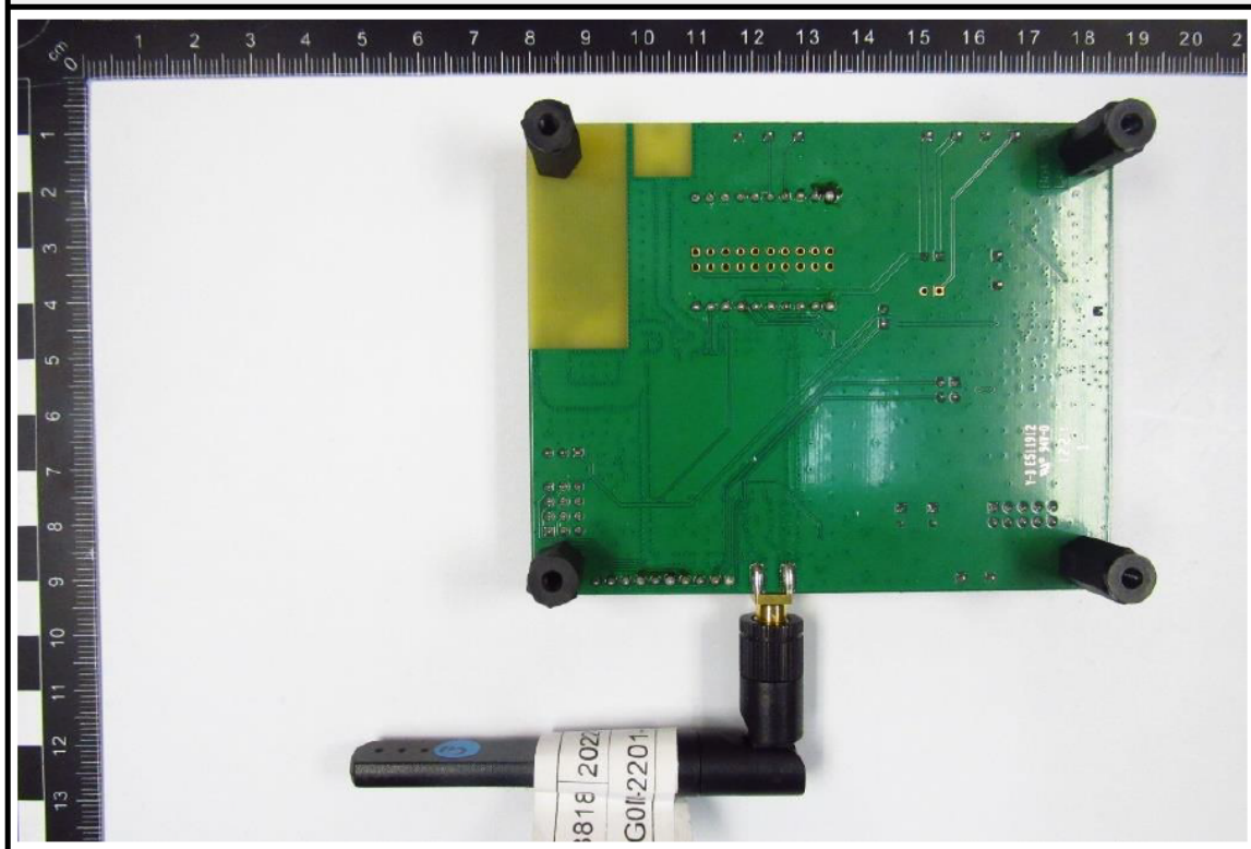
EUT Radiated Sample Bottom View
