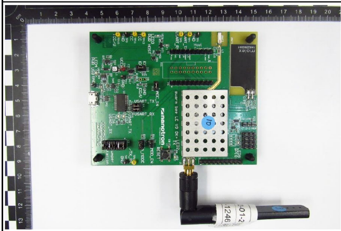
EUT Radiated Sample Top View
