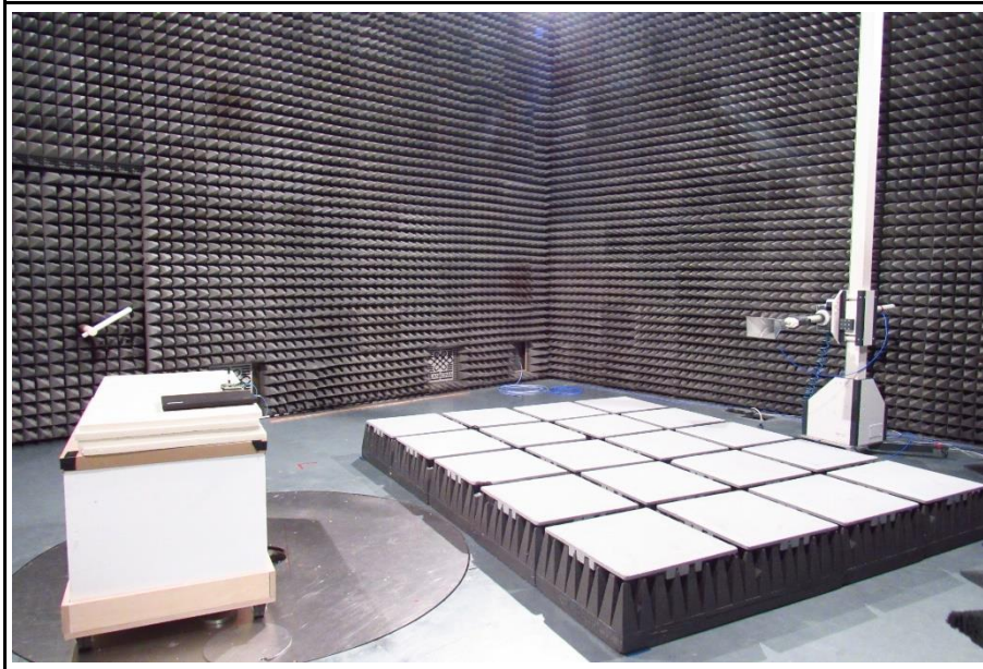
Radiated Setup above 1 GHz
