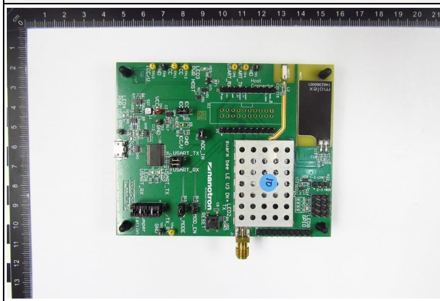
EUT Conducted Sample Top View
