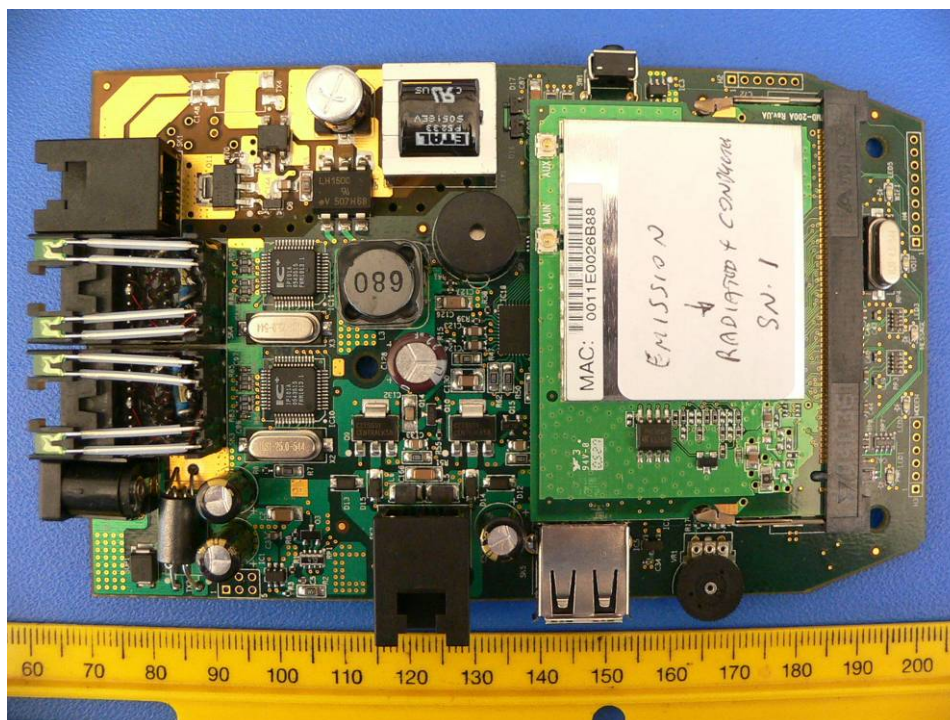
EUT – Main PCBA Component View
