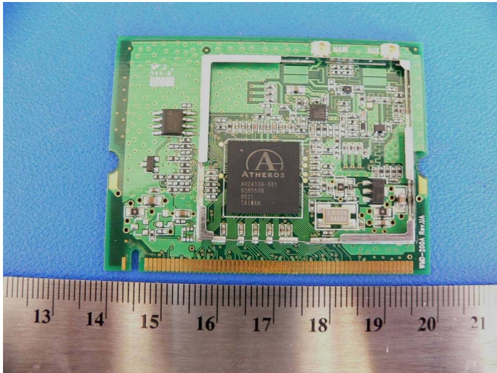
RF Board – with Shield Off
