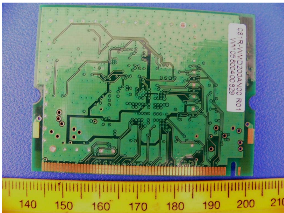
RF Board – Rear View
