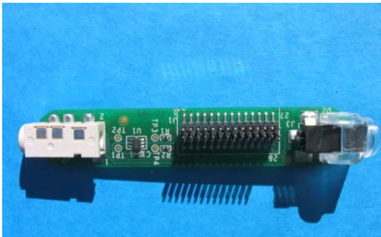
PC80189 Rev. B0 Assembly Top
