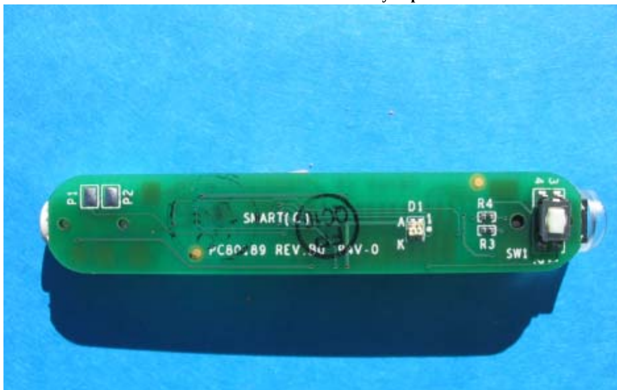
PC80189 Rev. B0 Assembly Bottom
