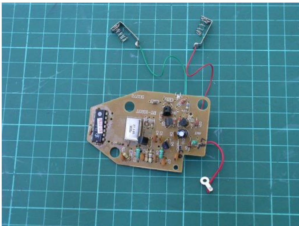
Photo 2: Interior photo of EUT (Base)
