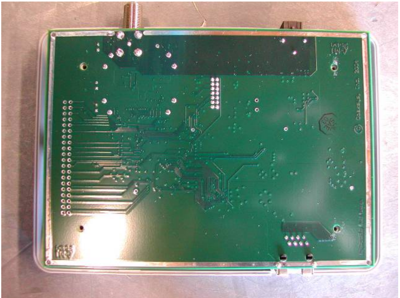
FIGURE 5: PLI Photograph Number 5406C3334SJ-14 illustrates the top view of the EUT with the bottom cover removed showing the circuit side of the EUT printed circuit assembly, number PN-00057 Rev. 3. [Short term confidentiality requested for this photo in FCC submission]
