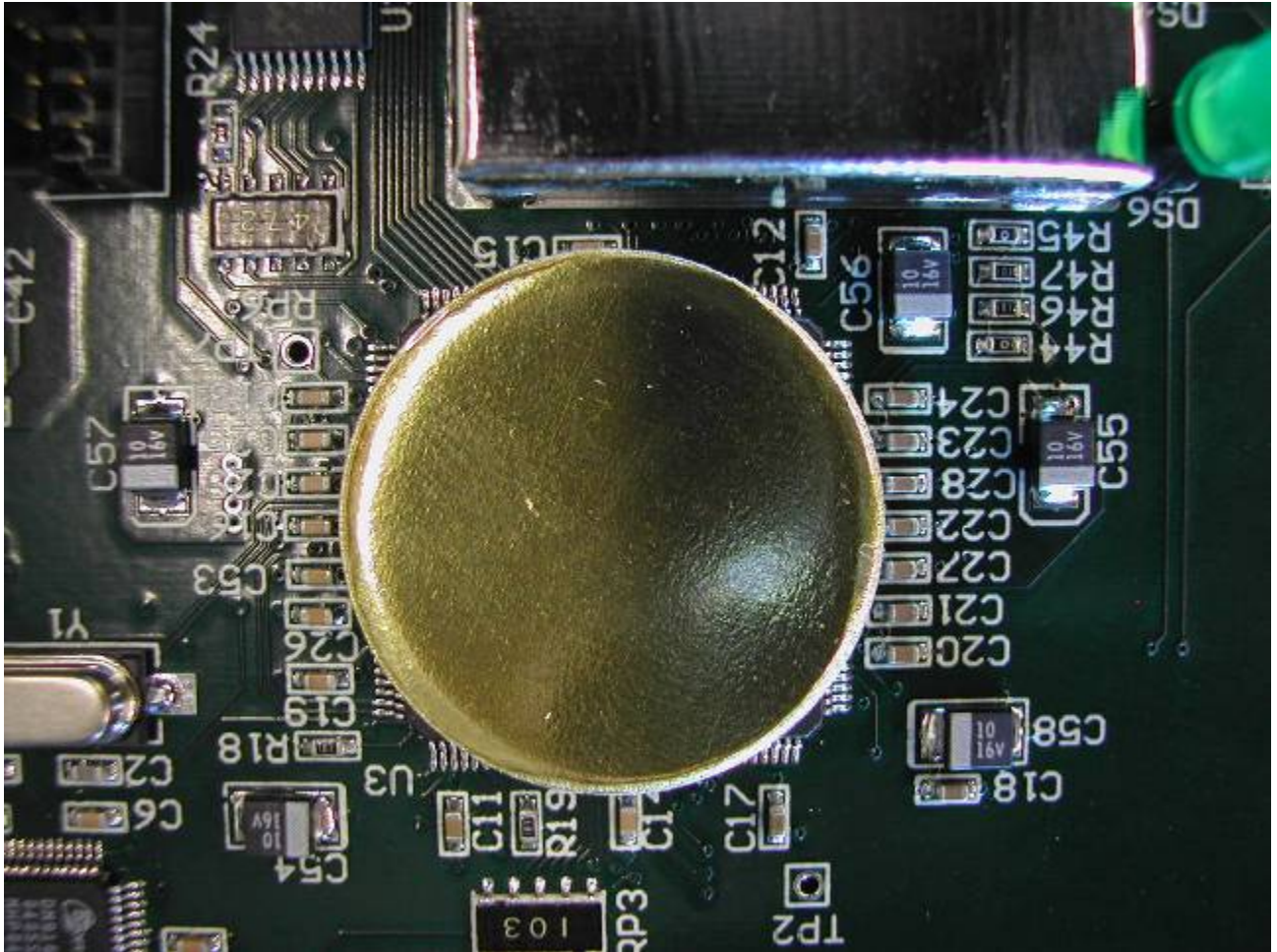
FIGURE 8: PLI Photograph Number 5406C3334SJ-13 illustrates a close up view of the RFDisc placed on top of “U3”. [Short term confidentiality requested for this photo in FCC submission]
