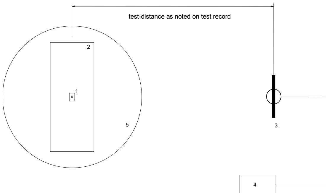
Figure 2: Example for measurement setup for radiated emission test below 30 MHz
