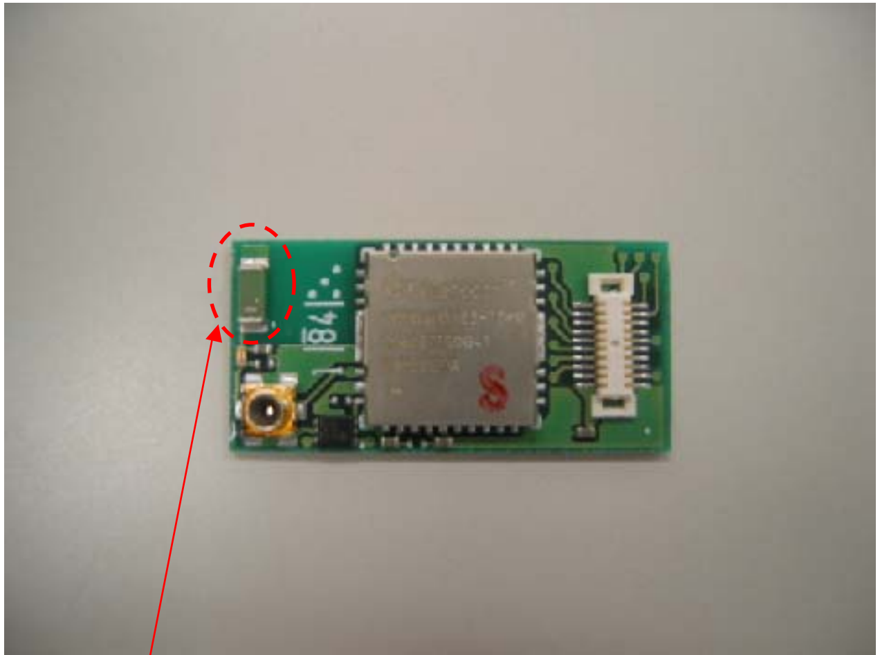
Bluetooth Antenna
