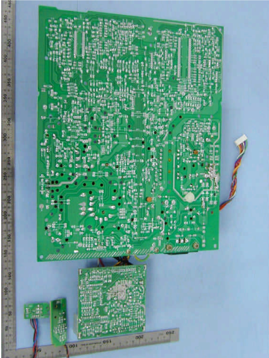
Solder Side View of Main Board
