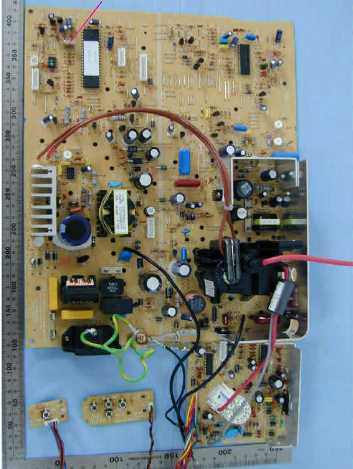
Component Side View of Main Board
