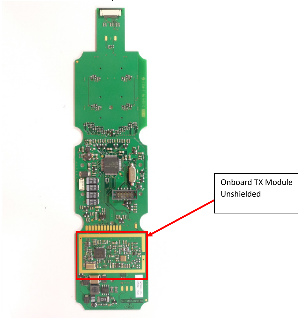
Mainboard – Top View without Shield
