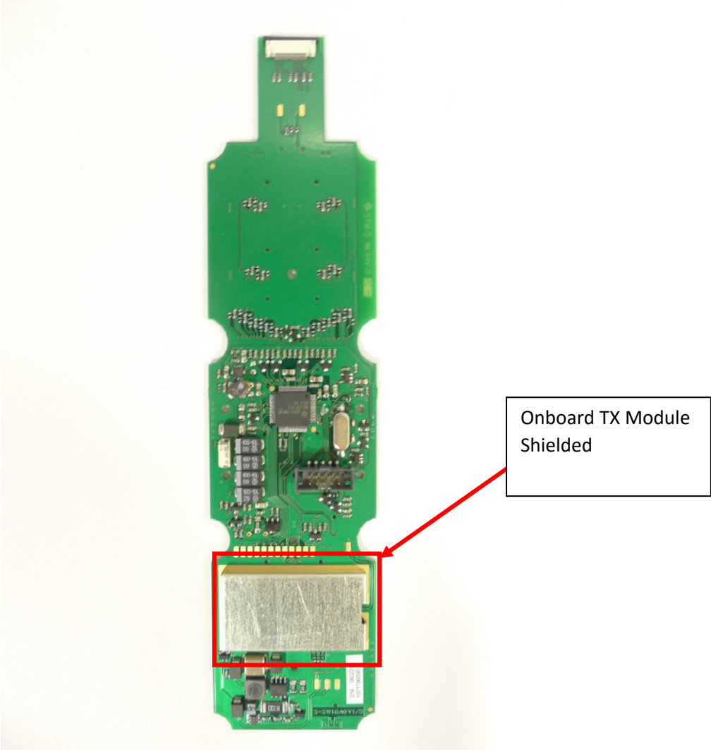
Mainboard – Top View with Shield
