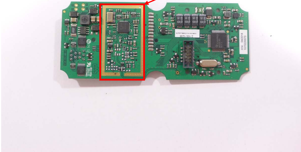
Mainboard Top – With Shield
