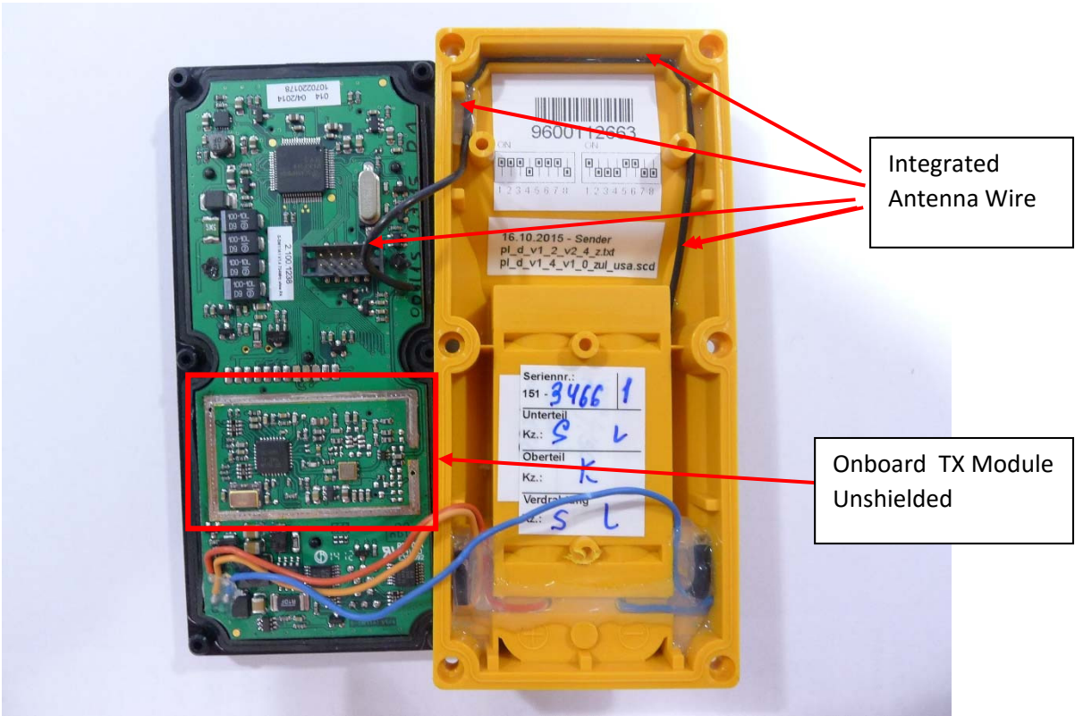
Internal Photos NBB Controls Inside
