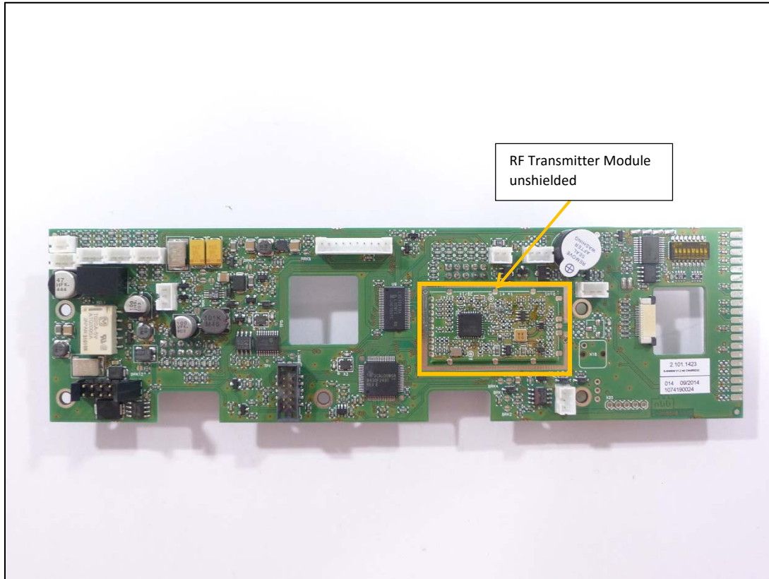
Mainboard – Top View without Shield
