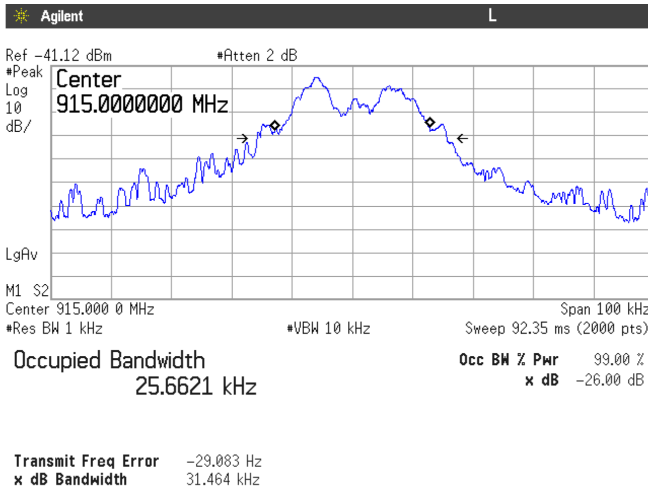
Figure 2: 99% Occupied Bandwidth, Low Channel
