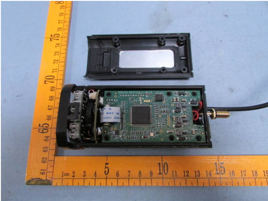
Model CA641 - Internal View
