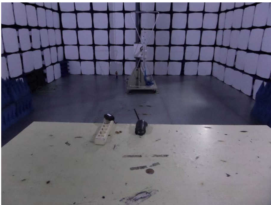
30MHz-1GHz
