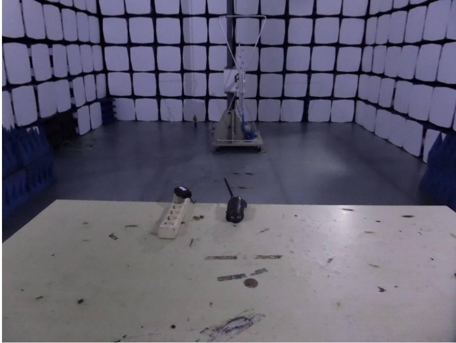
30MHz-1GHz
