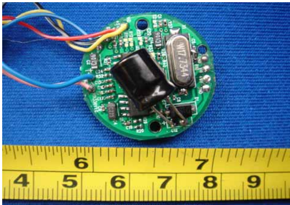
PCB 3- Solder View
