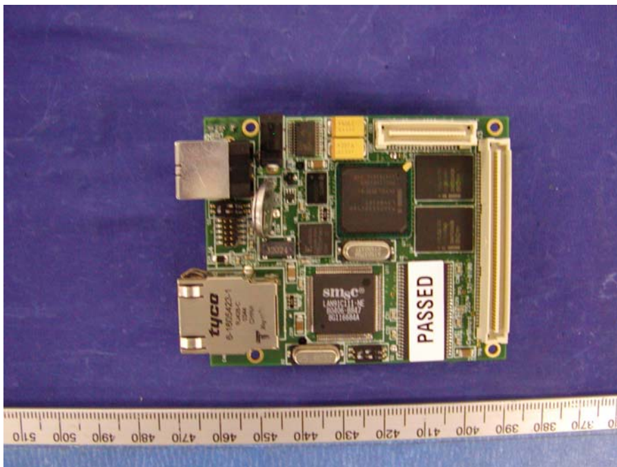
Component Board – Bottom View
