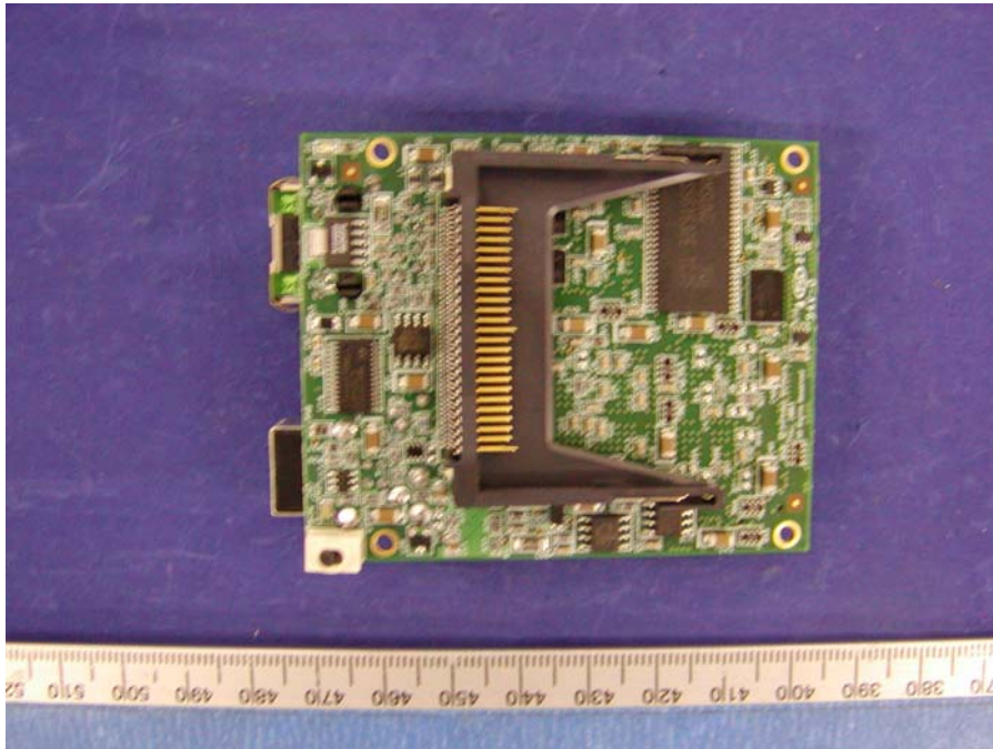
Component Board – Top View
