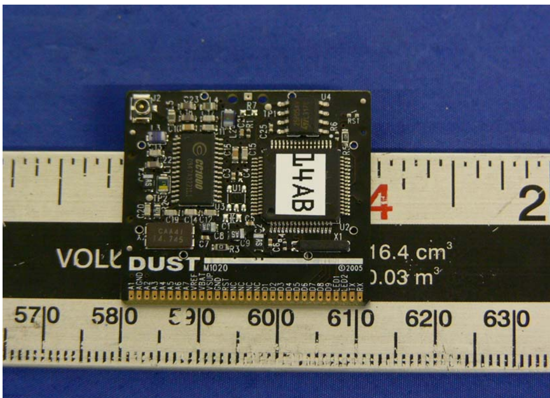
TX Component View
