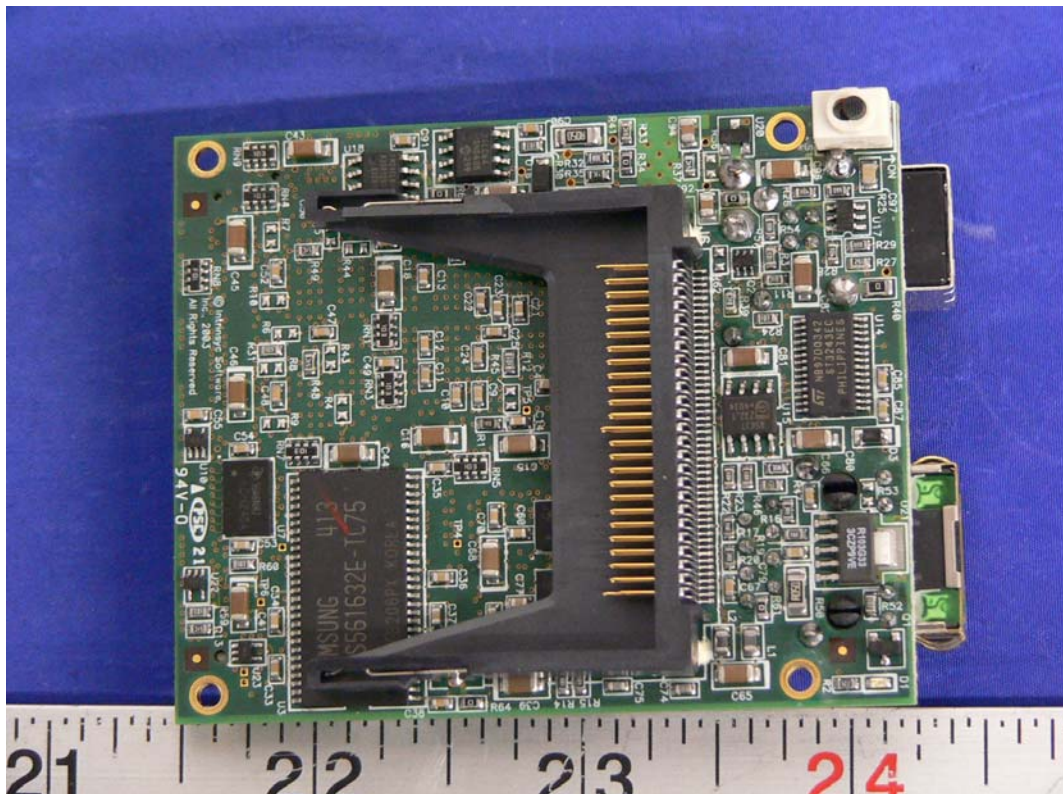
Top Board Component View
