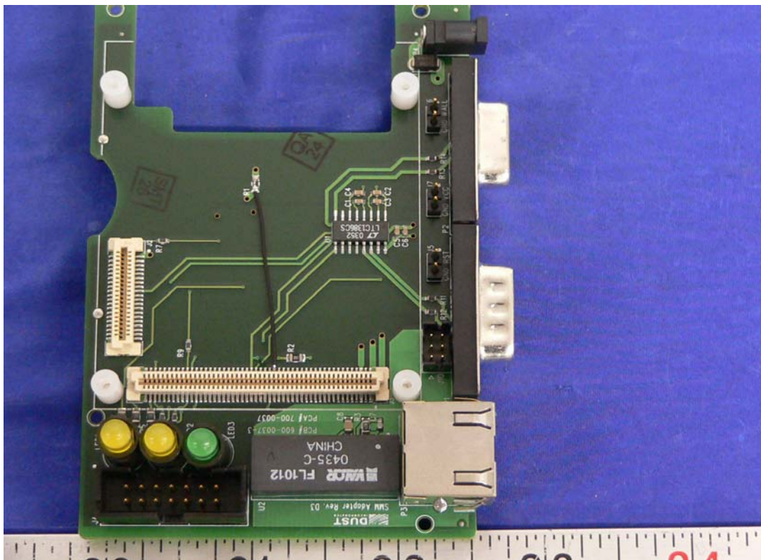
Bottom Board Component View
