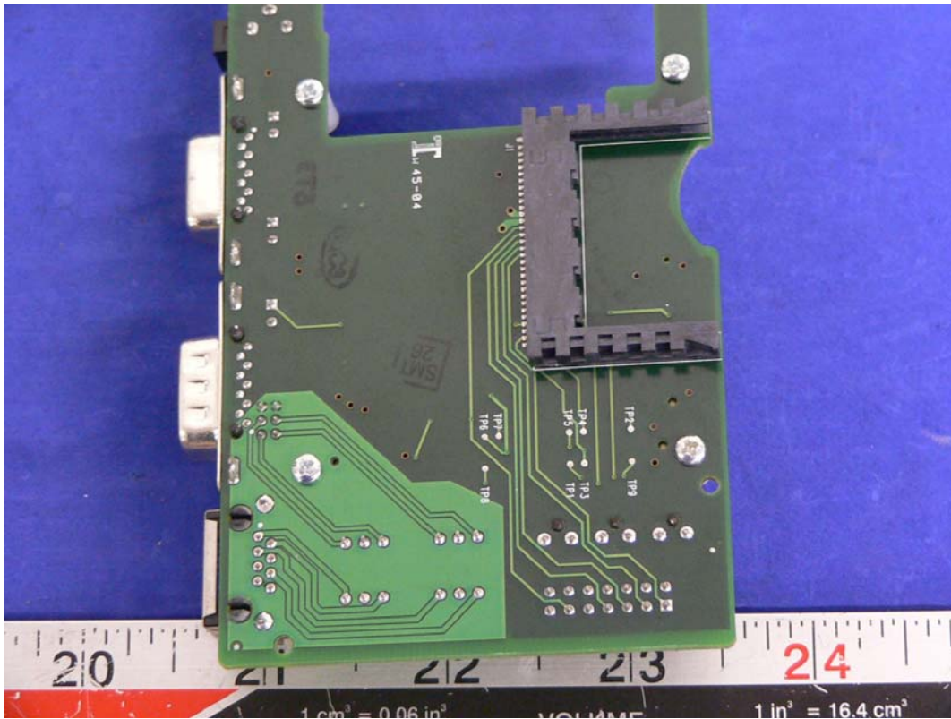
Bottom Board Solder View
