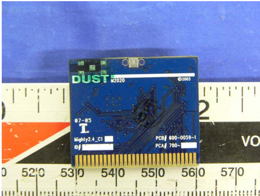
Transmitter – Solder View
