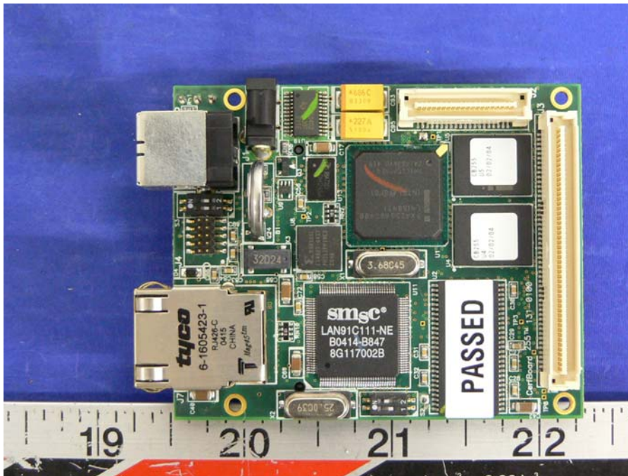
Top Card – Solder View
