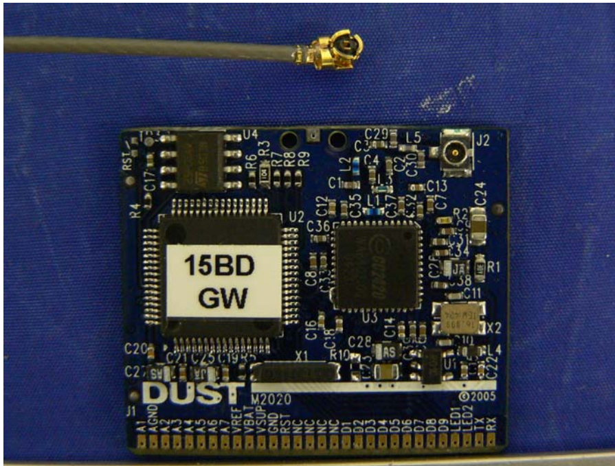
Antenna Connector View 2
