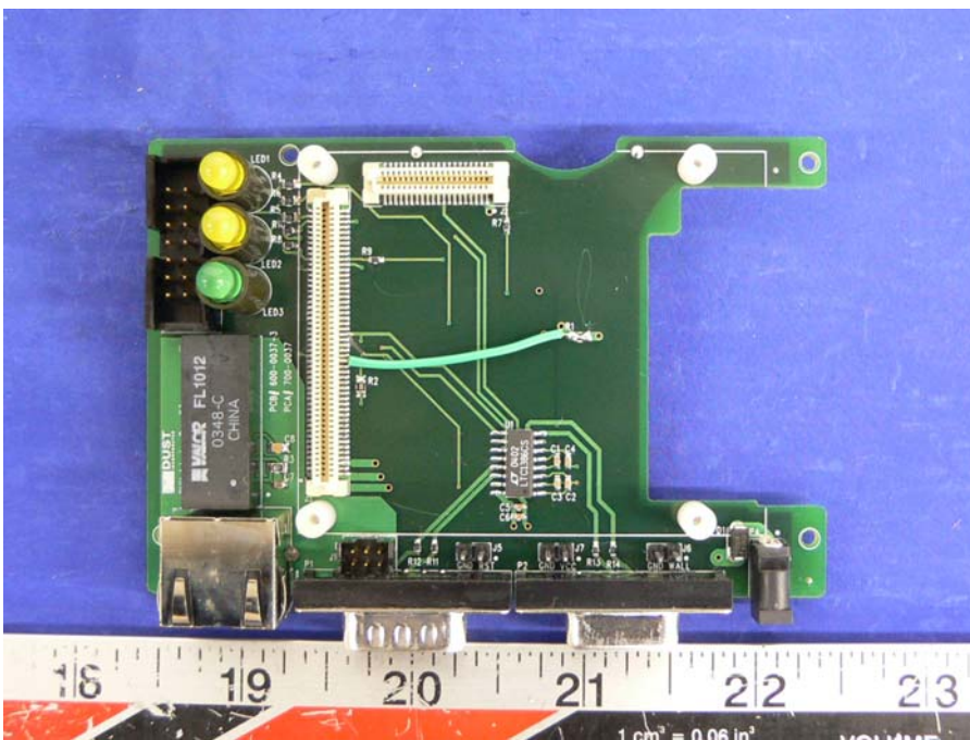
Bottom Card – Component View
