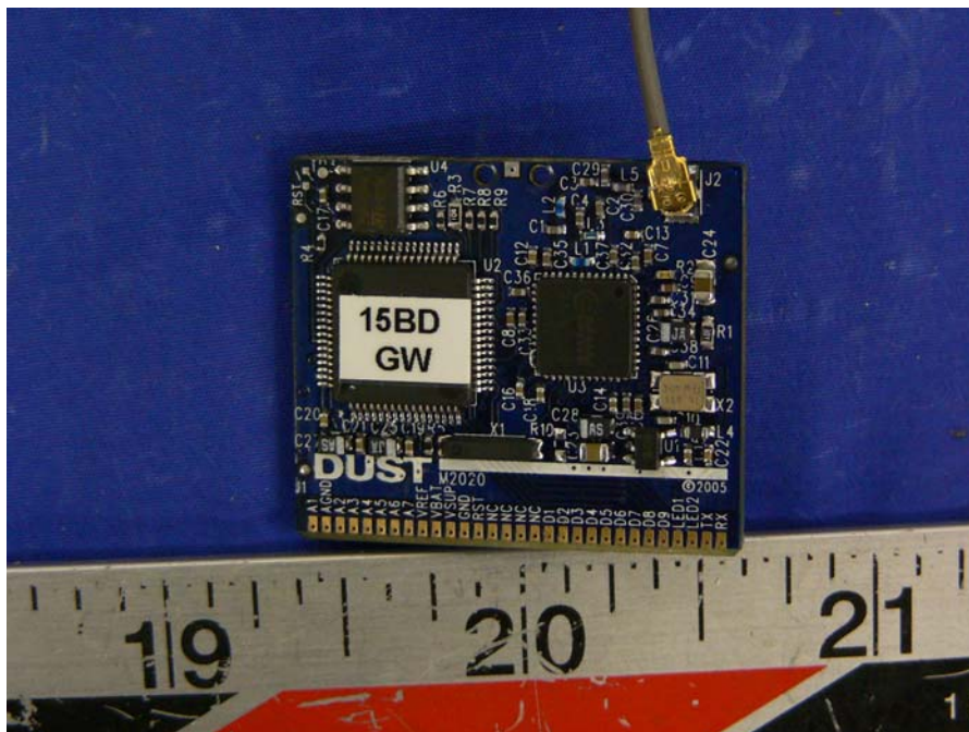
Antenna Connector View 1
