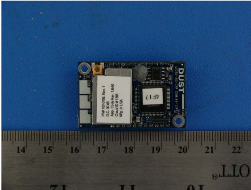
EUT – Component Side View without shielding off
