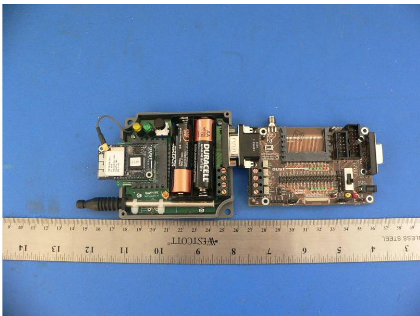
EUT - Built in the support tool View
