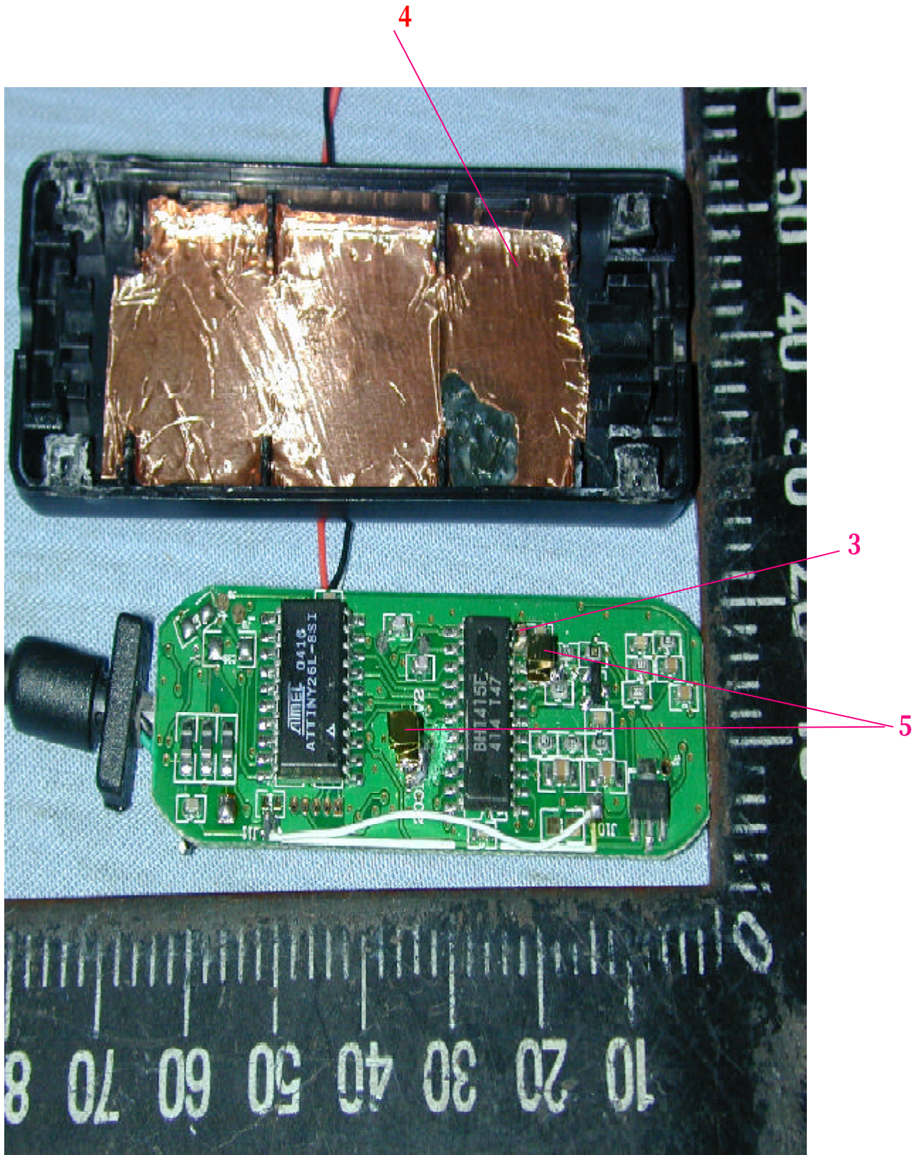
Solder Side View of Main Board 1
