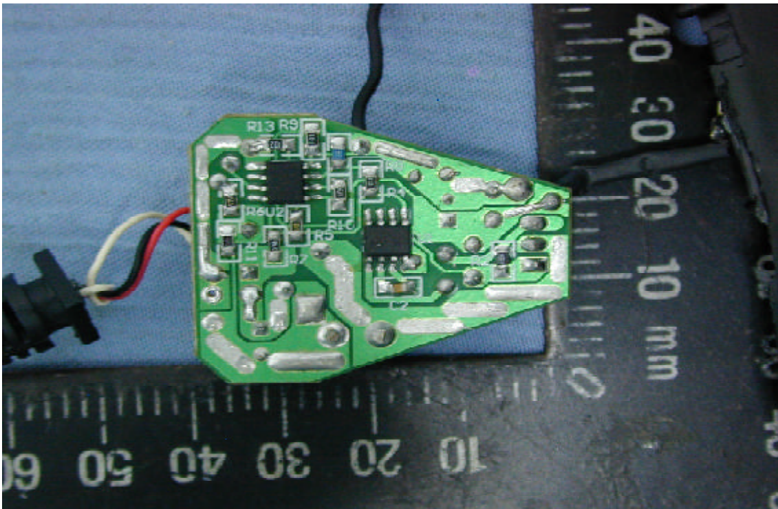
Solder Side View of Main Board 2
