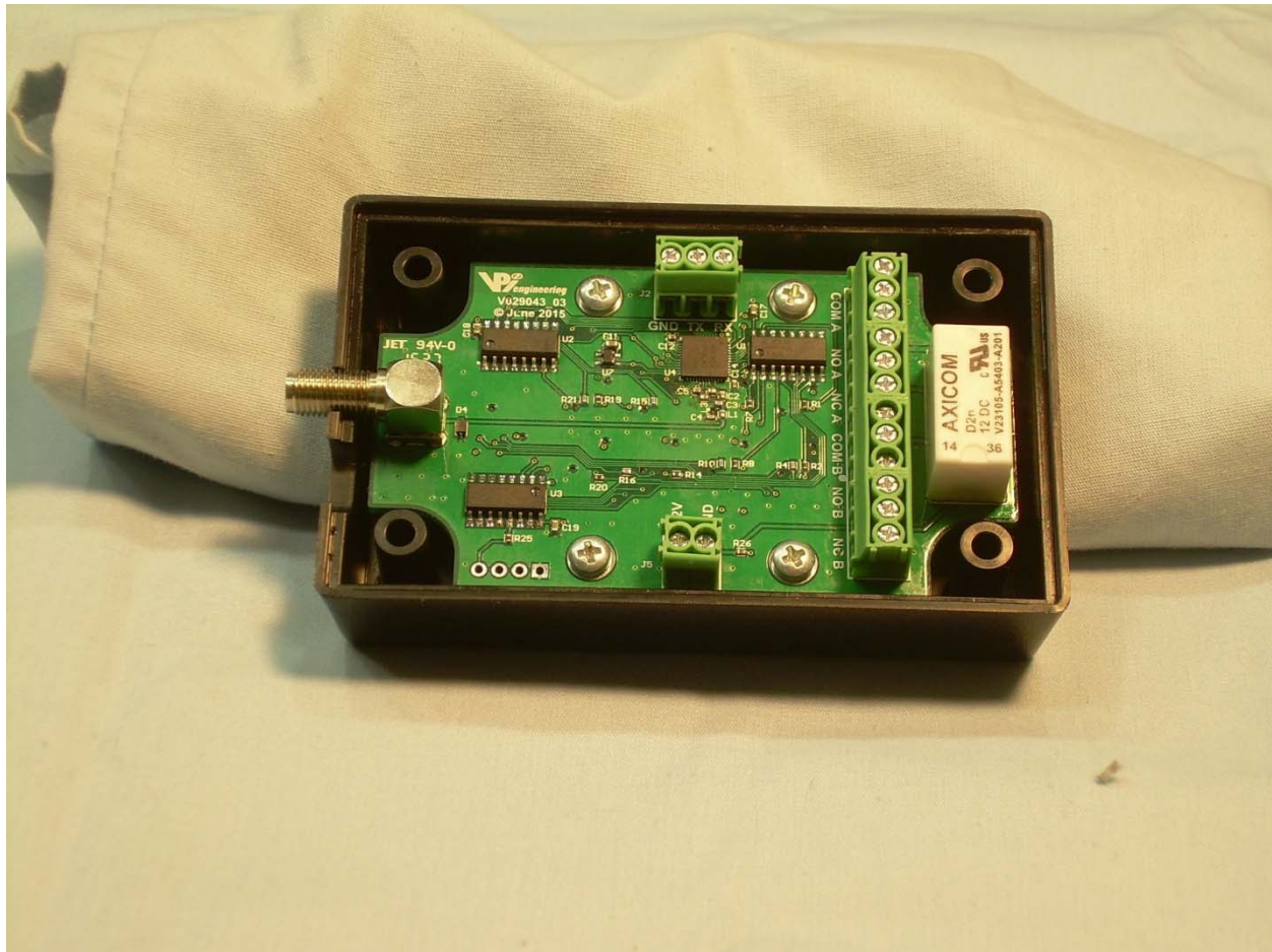
Photograph 5 – Back View of the EUT PCB
