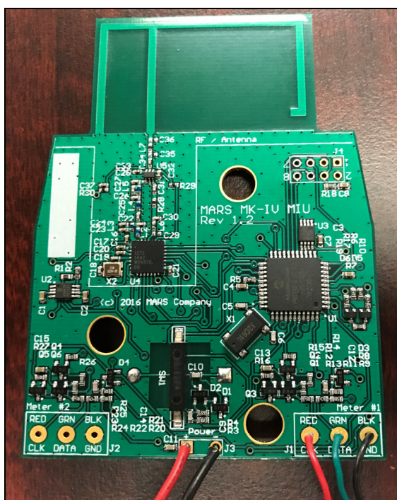
Figure 4: Internal Photo – PCBA Component
