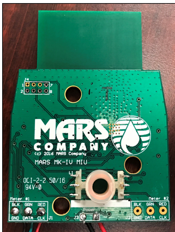
Figure 3: Internal Photo – PCBA Back
