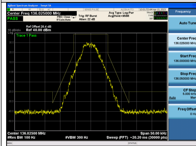
Emission Mask D@173.975MHz-7W-4FSK
