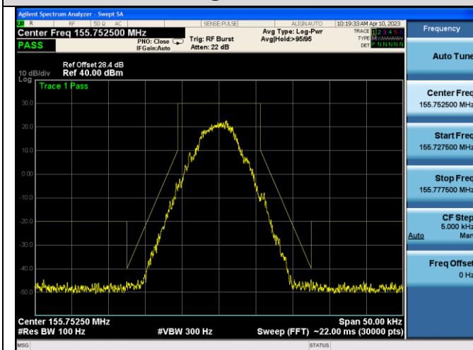
Emission Mask D@155.7525MHz-1W-4FSK
