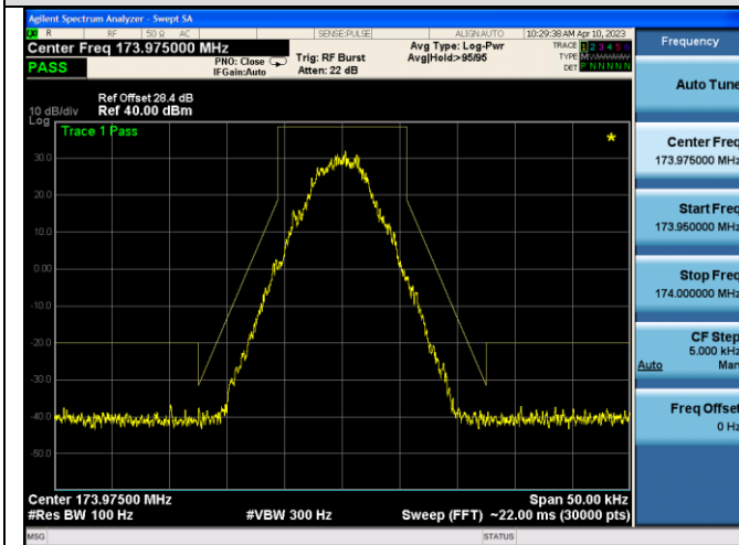
Emission Mask D@155.7525MHz-1W-4FSK
