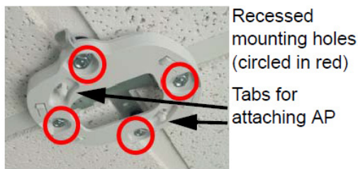
AP Mounting Plate (front, mounted)
