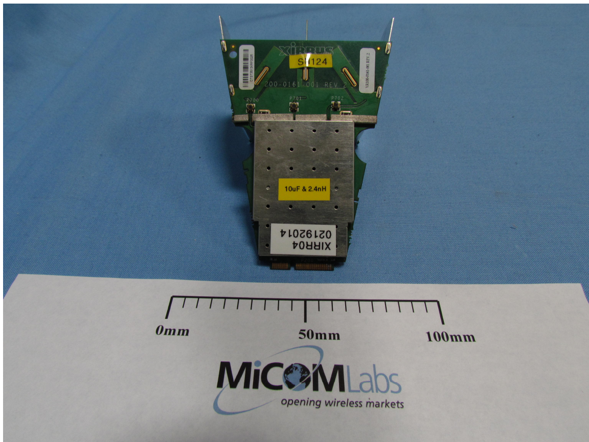
EUT Front with shield
