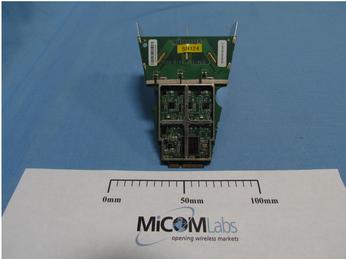
EUT front without shield
