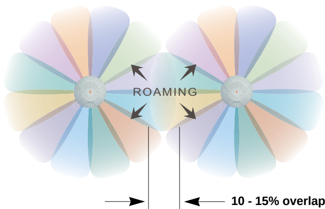
Figure 15. Overlapping Cells
