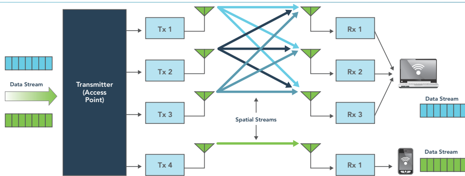
Figure 19. MU-MIMO with Four Antennas
