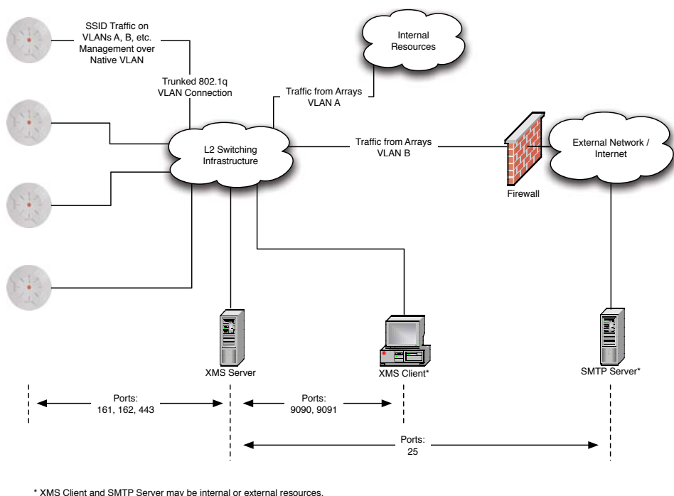
Figure 25. Port Requirements for XMS
