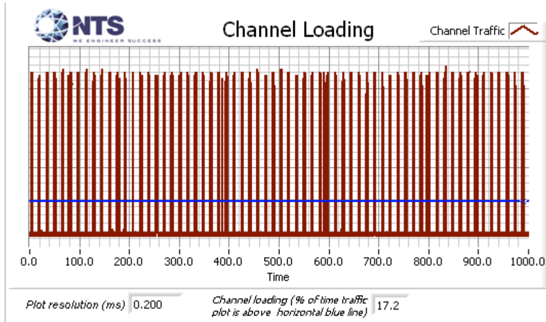
Figure 9 Channel Utilization During In-Service Detection Measurements (ac20 mode)
