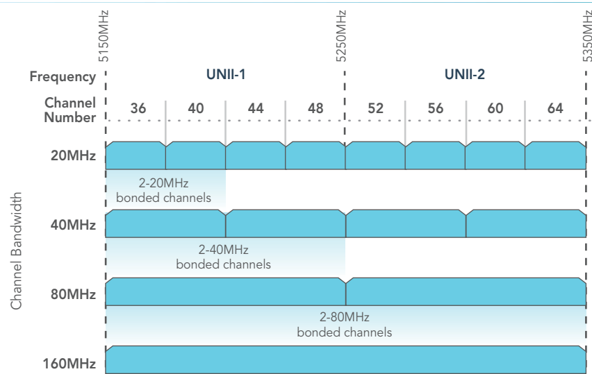
Figure 22. Channel Bonding (Channels 36-64 shown)
