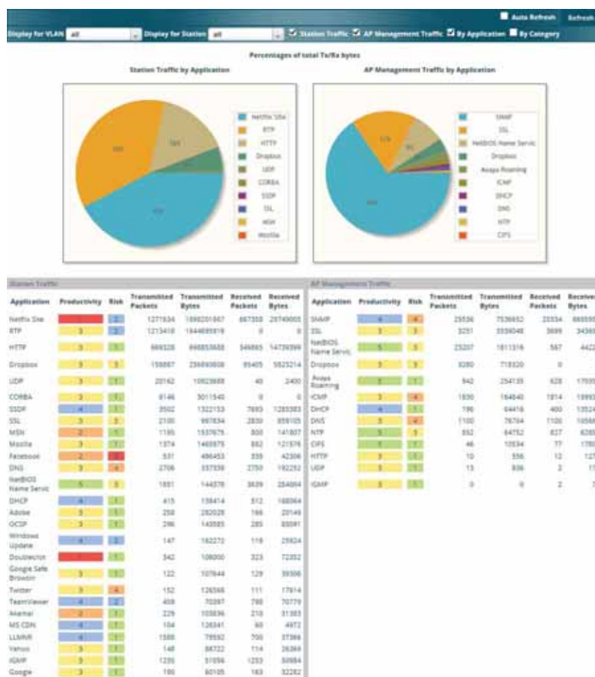
Figure 91. Application Control
