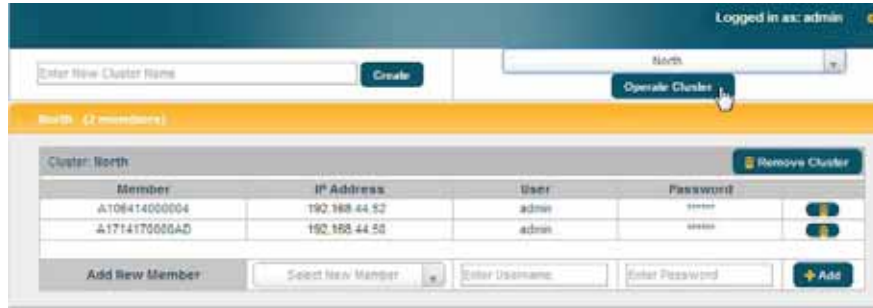
Figure 194. Cluster Management
