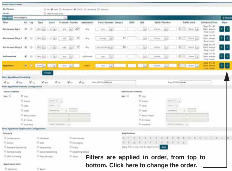
Figure 191. Filter Management
