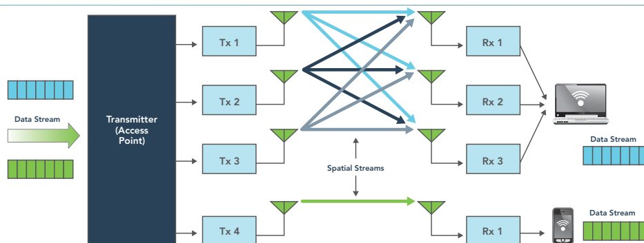
Figure 20. MU-MIMO with Four Antennas
