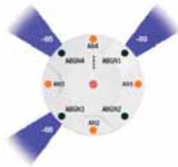
Figure 78. Station Noise Floor Values—Colorized Graphical View
