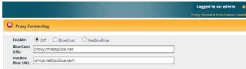
Figure 123. Proxy Forwarding
