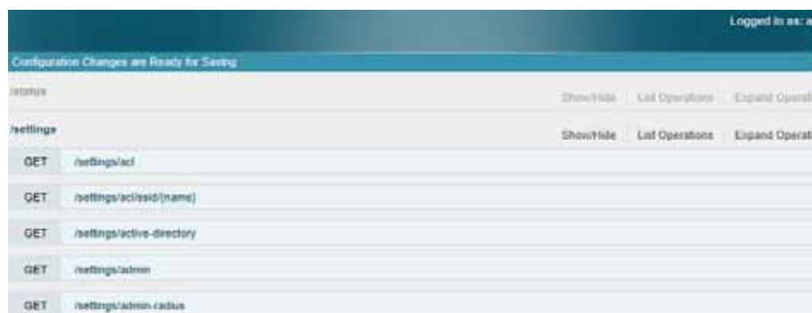
Figure 206. API Documentation
