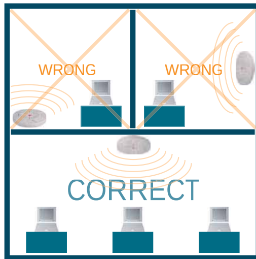
Figure 31. AP Placement
