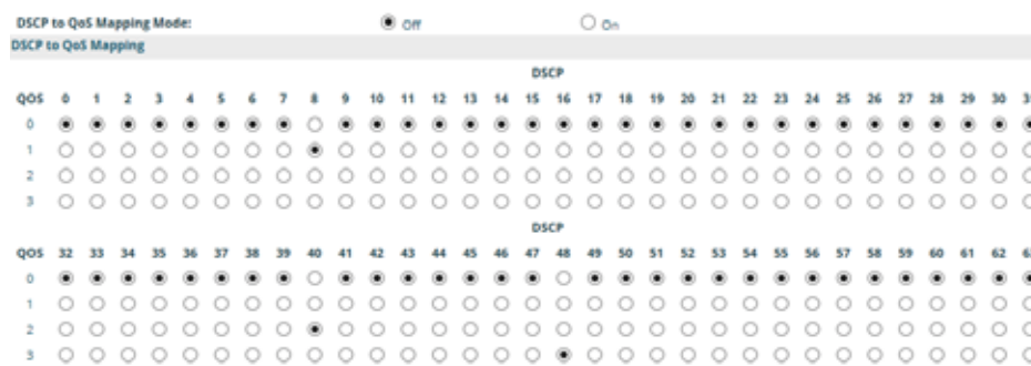
Figure 184. DSCP Mappings
