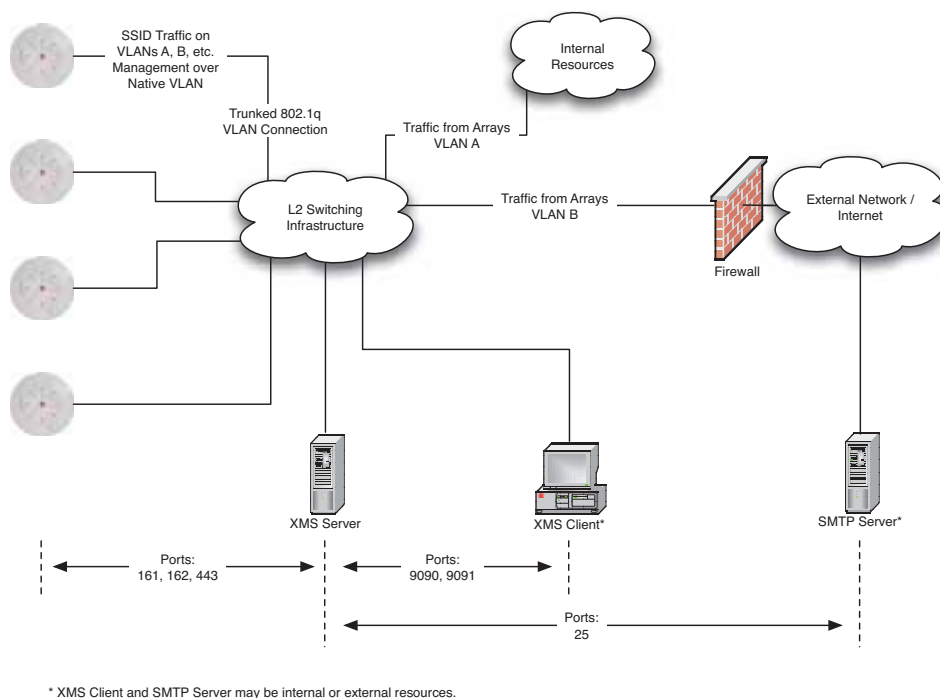
Figure 26. Port Requirements for XMS
