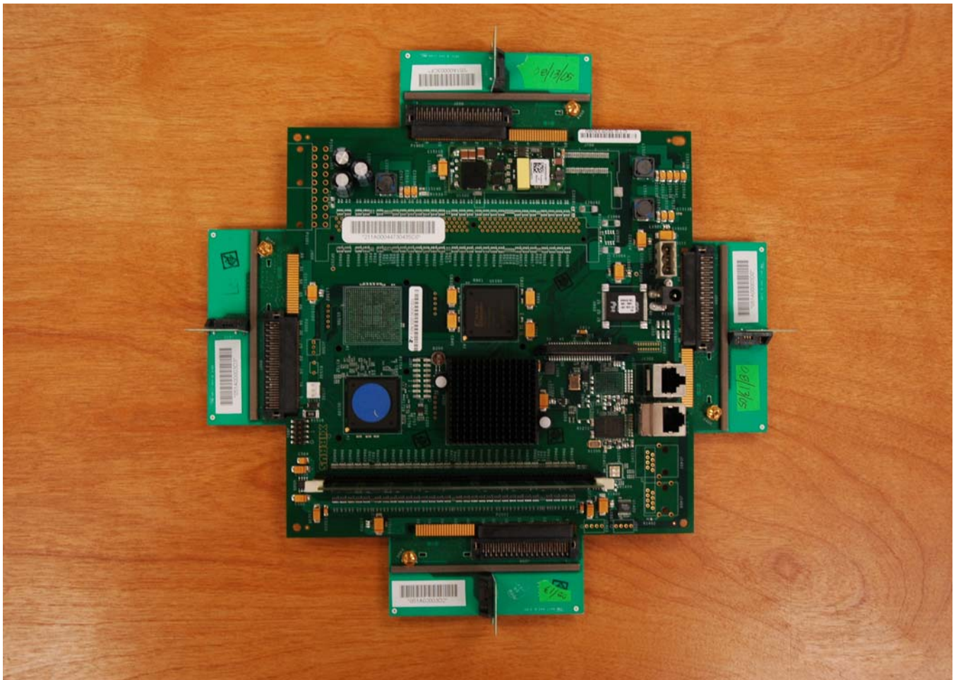
Main Processor Board (Top/Bottom) with radio interface boards connected
