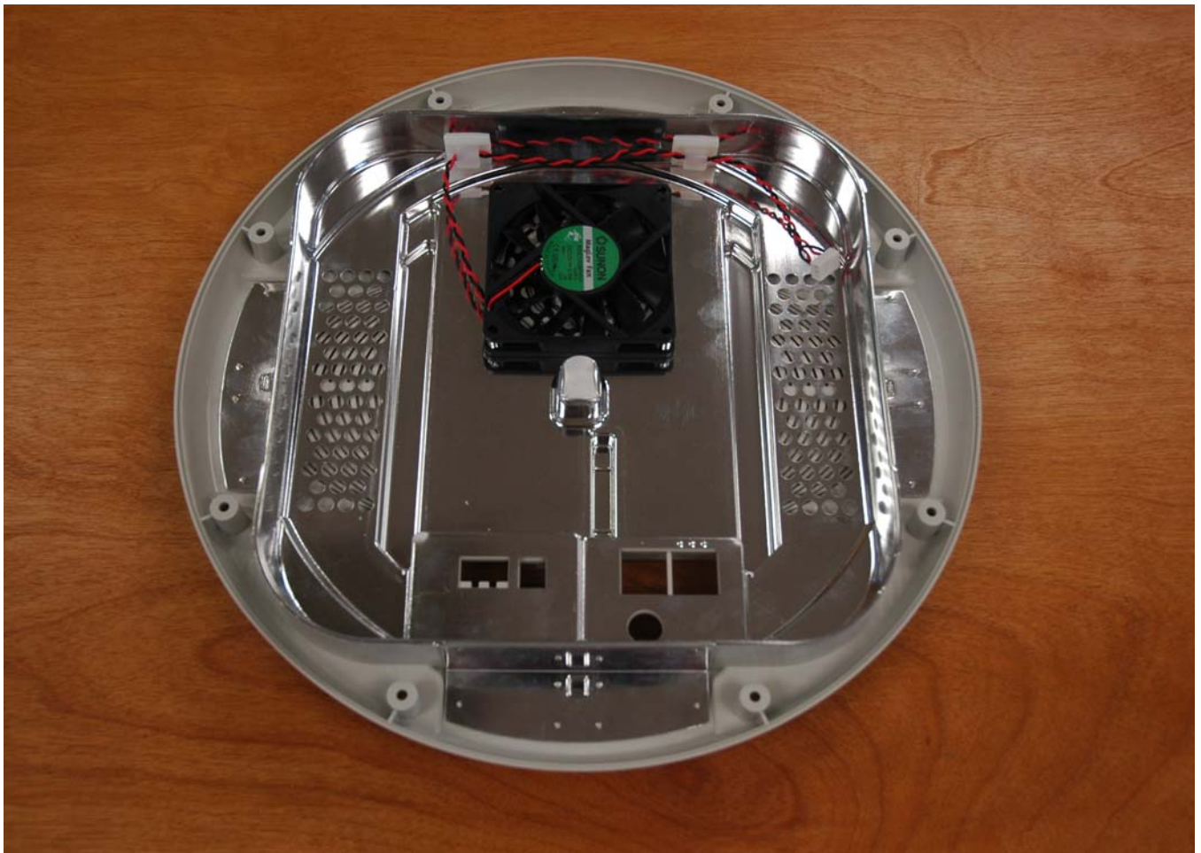
Internal View - top/bottom shields
