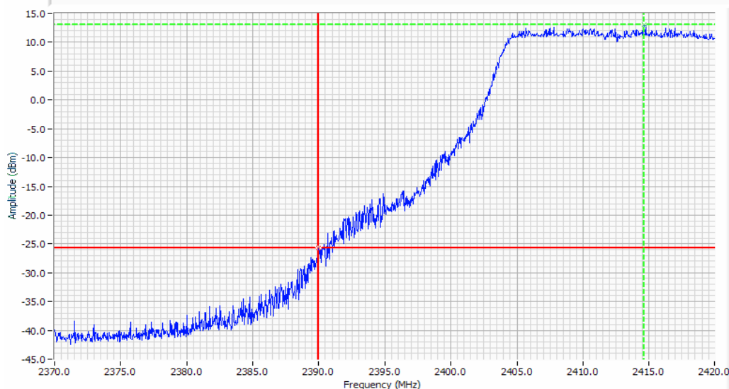
Band Edge delta using RB=VB=1MHz
