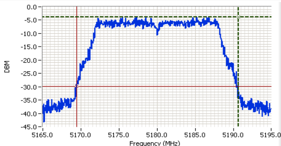
PSD, 99% Bandwidth and Power Over Span Plot
