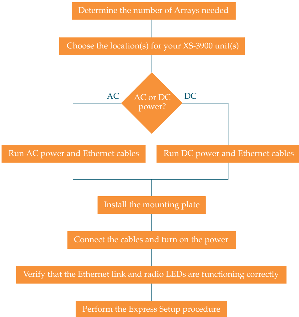
Figure 24. Installation Workflow
