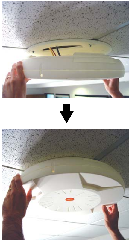
Figure 28. Attaching the Unit
