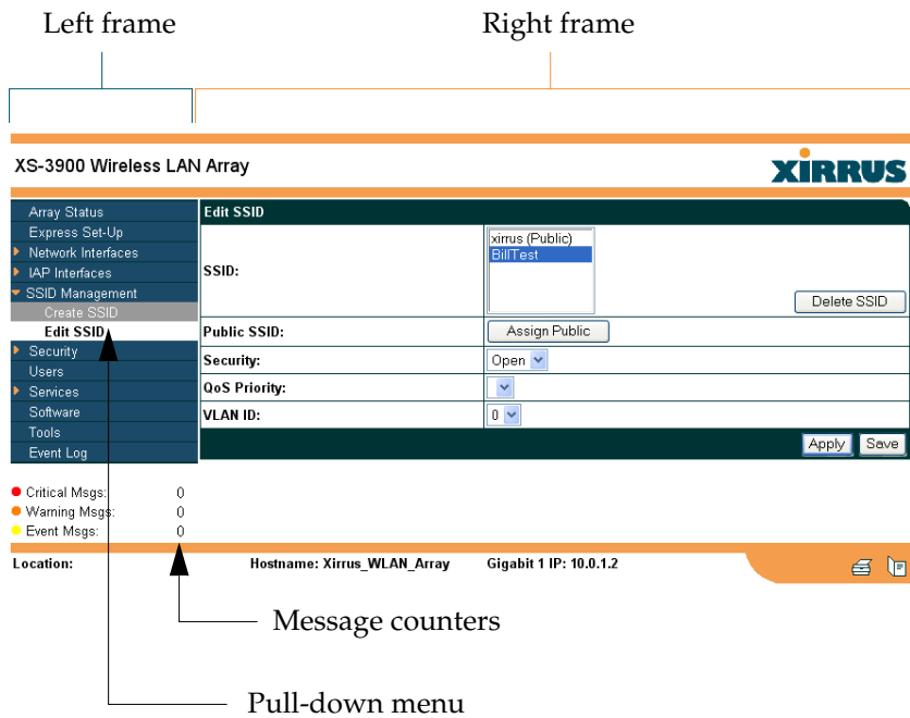
Figure 37. WMI: Frames
