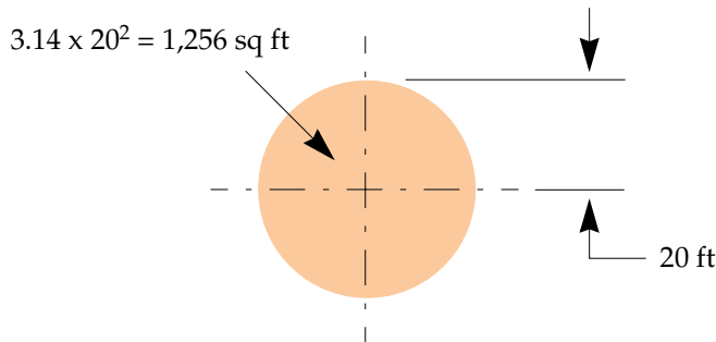
Figure 13. Calculating the Area of a Circle
